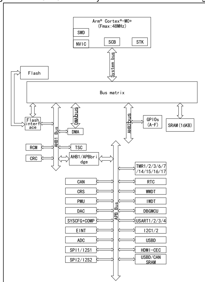
Figure 1 APM32A072xBTx System Architecture Block Diagram
