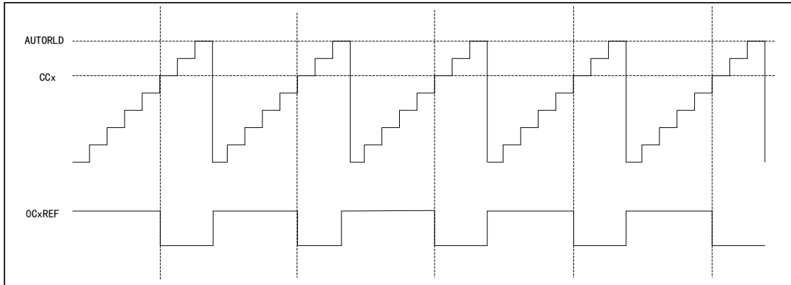
Figure 29 PWM1 Count-up Mode Timing Diagram
