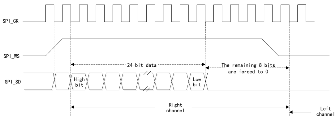
Figure 116 I2S Philips Protocol Waveform (24 bits)
