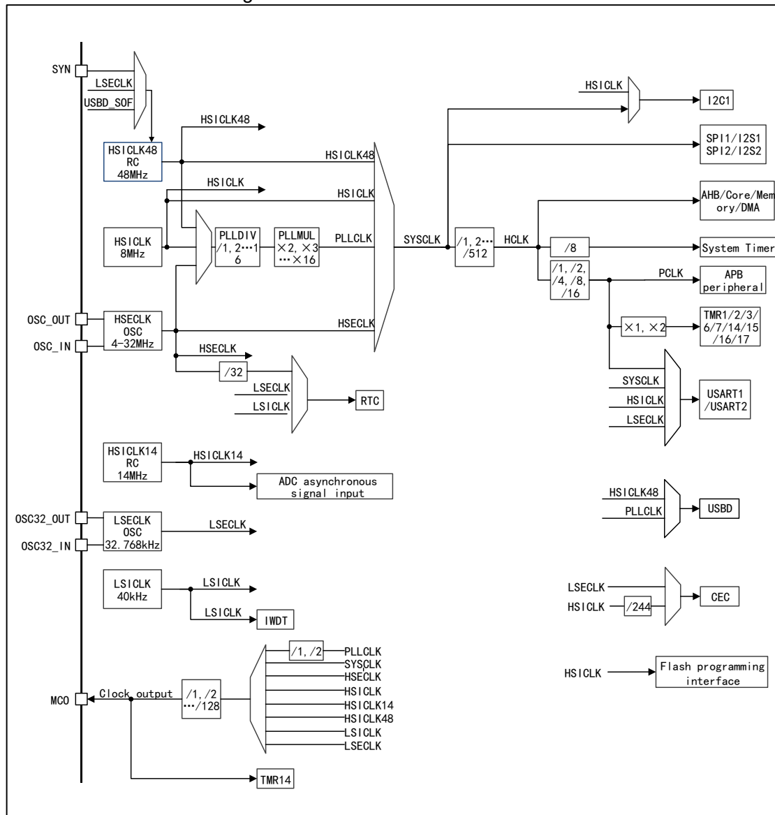
Figure 4 APM32A072xBTx Clock Tree
